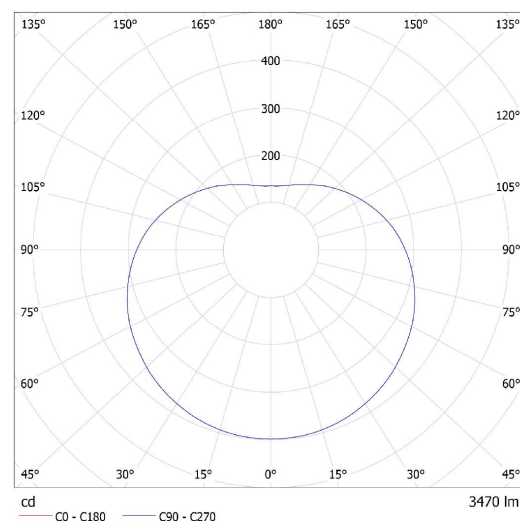
Lucis ZK.P1.400.X POLARIS ZK LED / LDC (Polar)
